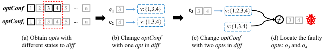
Fig. 4. Locate faulty optimization strategies in Fig. 3.
