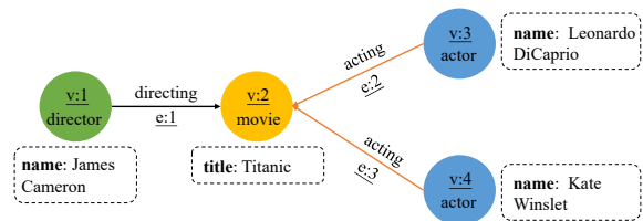
Fig. 2. A labeled property graph. We label each vertex and edge in the graph with unique IDs, e.g., v:1 represents a vertex with an ID 1.
